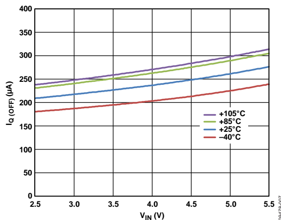
Figure 7. Typical Off Time Current ( I_{Q(OFF)} )
