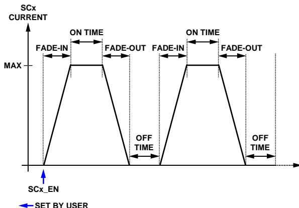
Figure 34. LEDx Blink Mode with Fading
