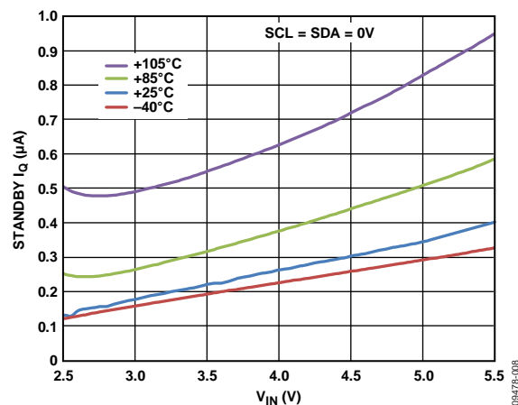
Figure 8. Typical Standby I_Q
