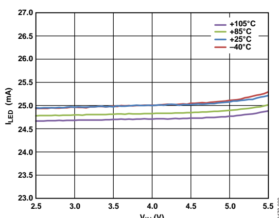
Figure 9. Typical Diode Current vs. V_{IN}
