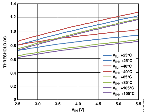
Figure 19. Typical I_C Thresholds, V_{IH} and V_{IL}
