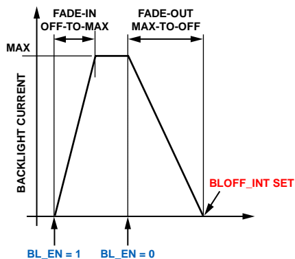
Figure 37. Backlight Off Interrupt Timing Diagram
