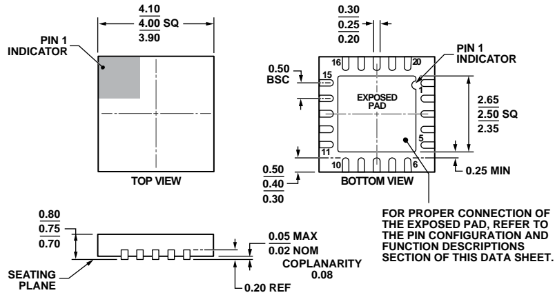
Figure 42. 20 Lead Lead Frame Chip Scale Package [LFCSP_WQ] 4 mm × 4 mm Body, Very Very Thin Quad (CP-20-10) Dimensions shown in millimeters
