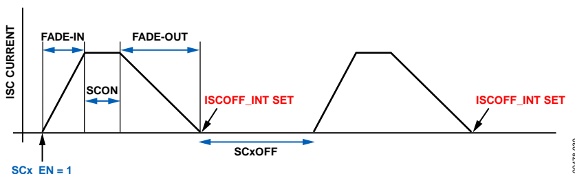
Figure 38. Independent Sink Off Interrupt Timing Diagram
