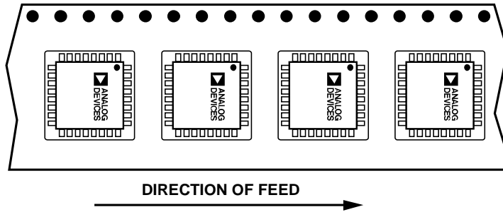
Figure 43. Tape and Reel Orientation for LFCSP Units
