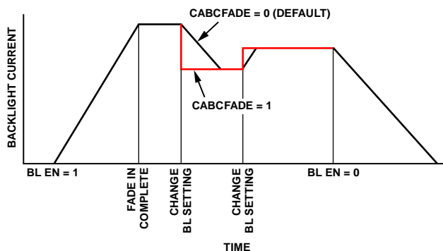
Figure 33. Effect of the CABCFADE Bit
